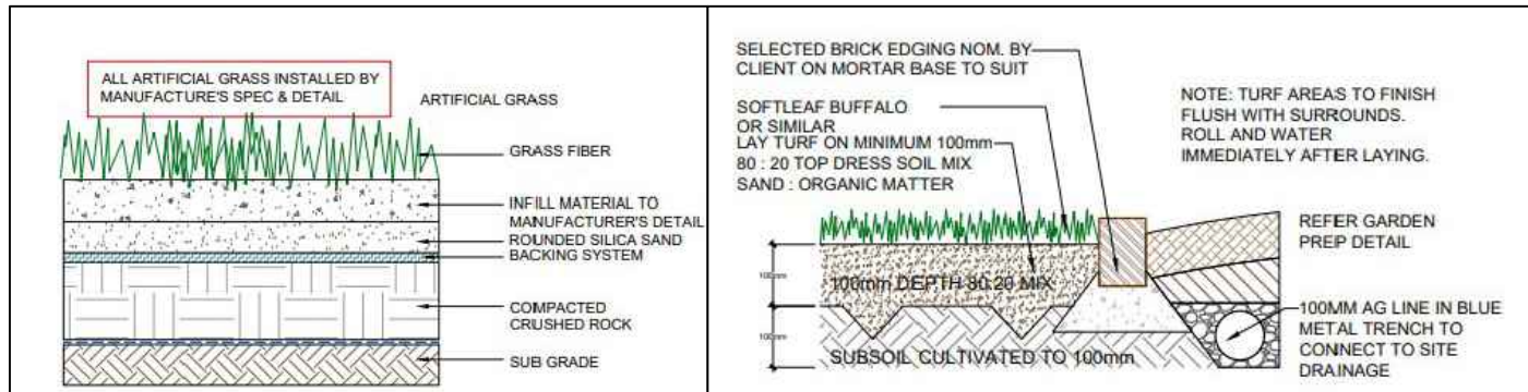
Artificial Grass Detail
