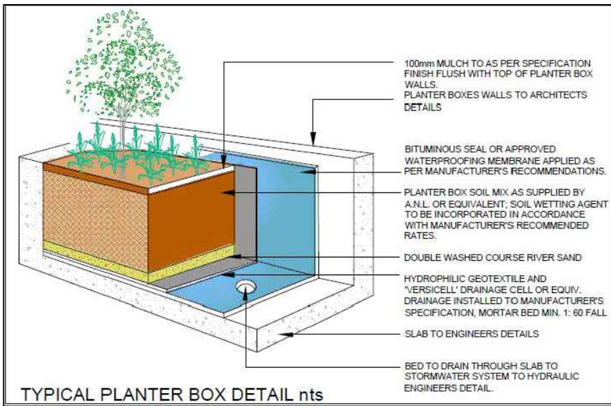
Typical Planter Box on Slab Detail
