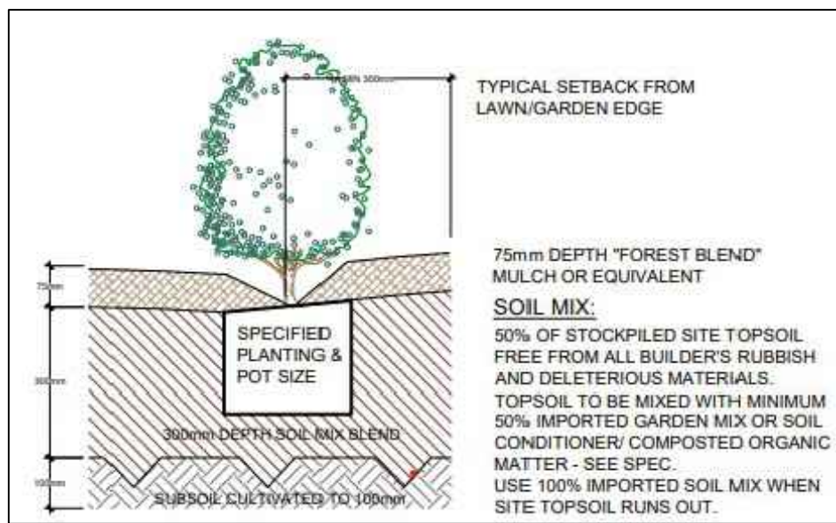
Typical Garden Preparation Detail
