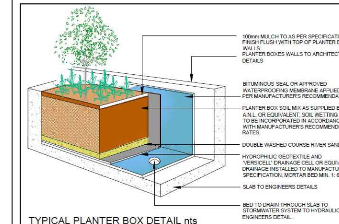
Typical Planter Box Detail nts
